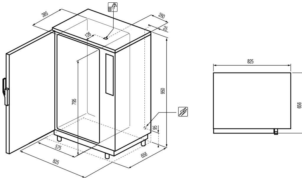
Model RRS101C (type RRS101C) – Nr. 10 GN 1/1
