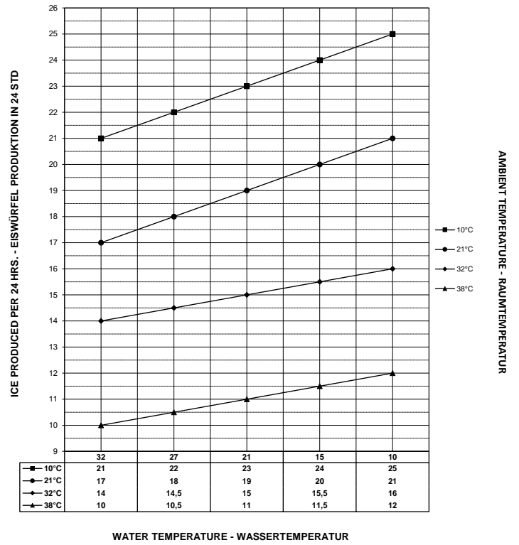
SDH 24 AIR COOLED MODELS - LUFTKÜHLUNG
