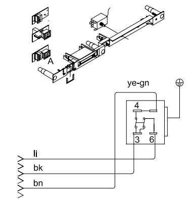
With mechanical thermostat and without light
