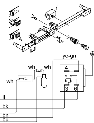
With mechanical thermostat and light
