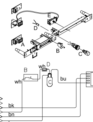
With electronic thermostat and light
