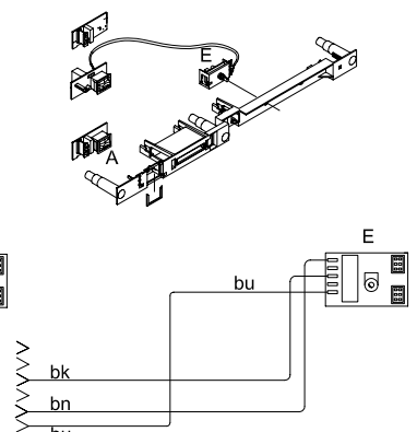
With electronic thermostat and without light
