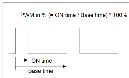
Fig. 1 Definition of the PWM (Heating output in %)
