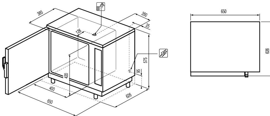
Model RRS040C (type RRS040C) – Nr. 4 GN 2/3
